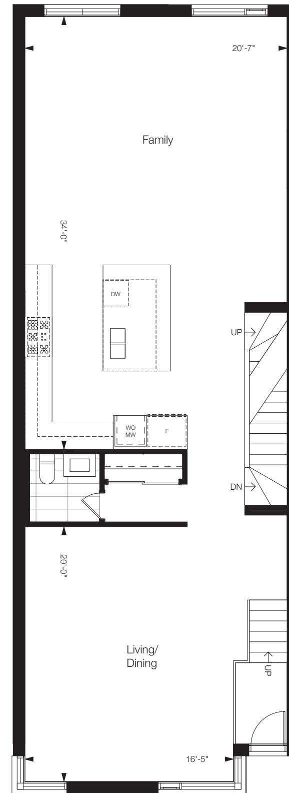
Main Floor
