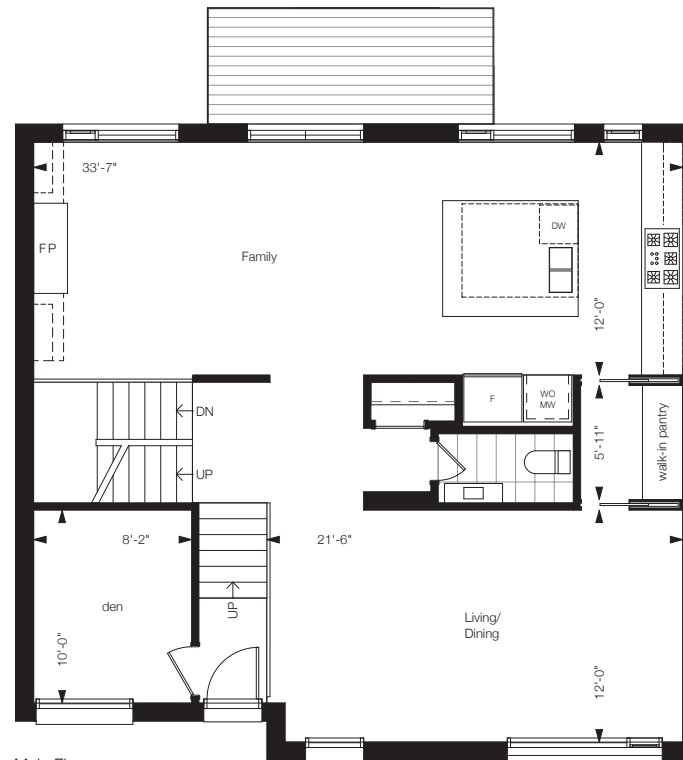
Main Floor
