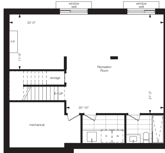
Basement
